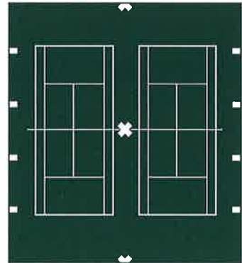
Layout #4 Narrow Court Club/Tournament
